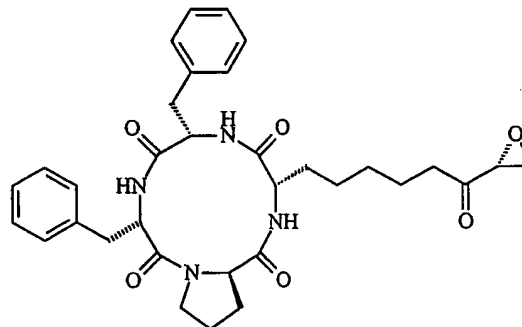
Trapoxin B
